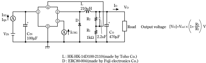
Fig. 1 Test Circuit
